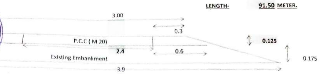
SECTIONAL ELEVATION
